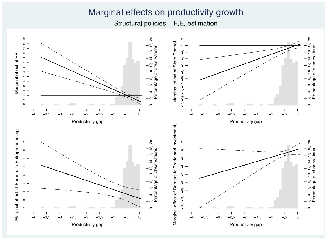
Figure 1: Marginal effects of structural reforms, OLS
